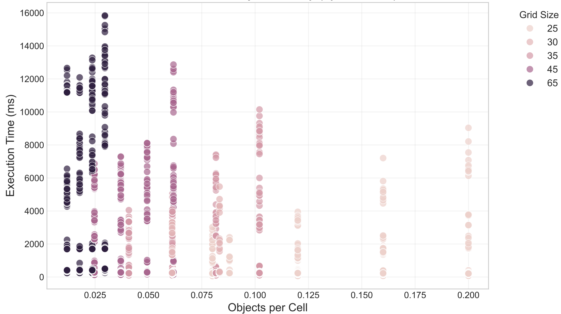
Performance vs Object Density (by Grid Size)
